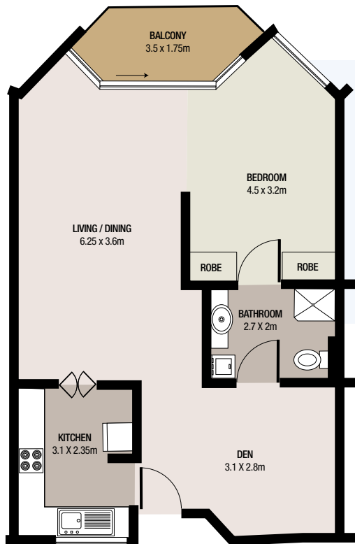
B Type unit 75.6m 2 (incl. balcony)
